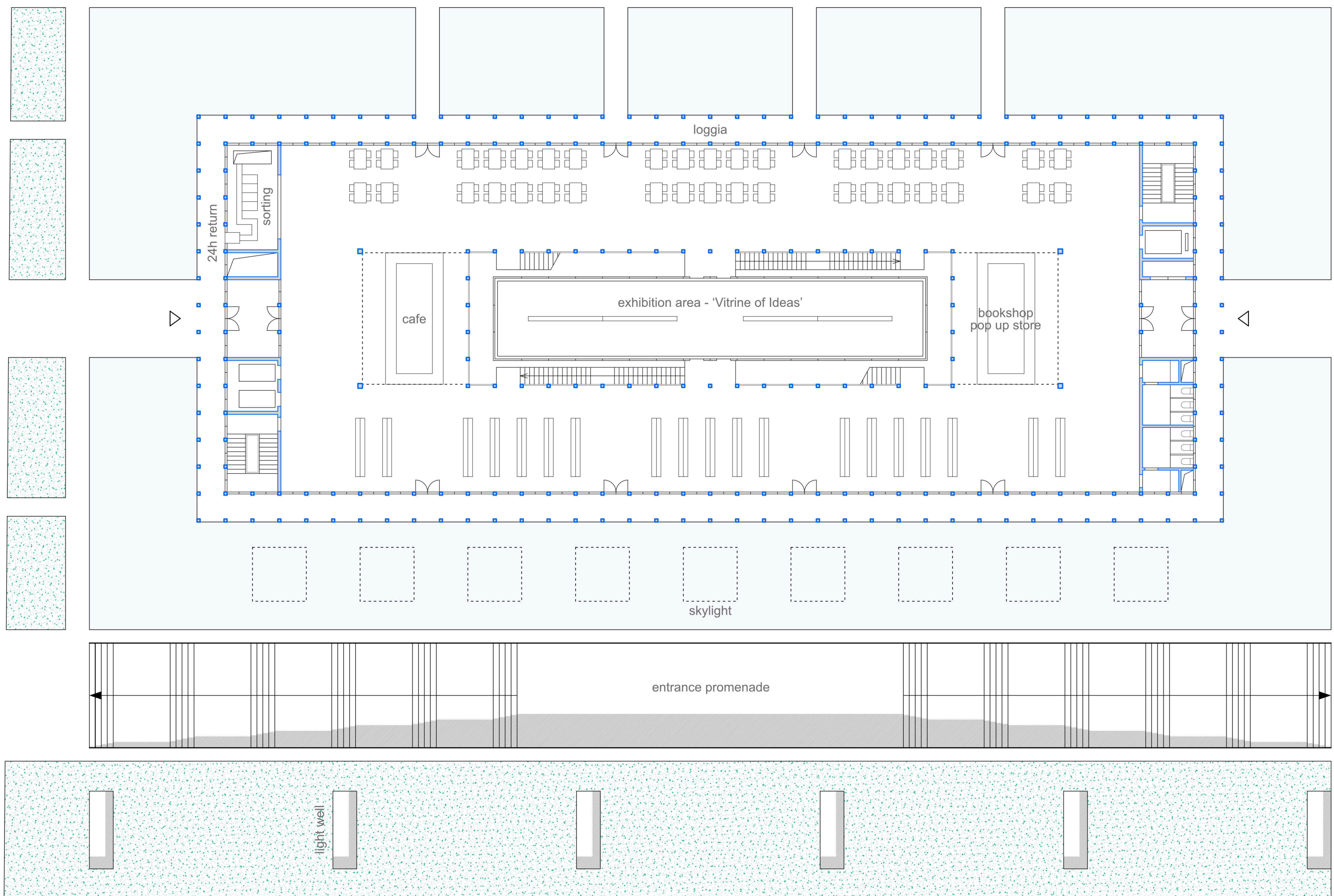
Ground Floor - Entrance Area (newspapers, magazines, café, pop-up store) 1:200
