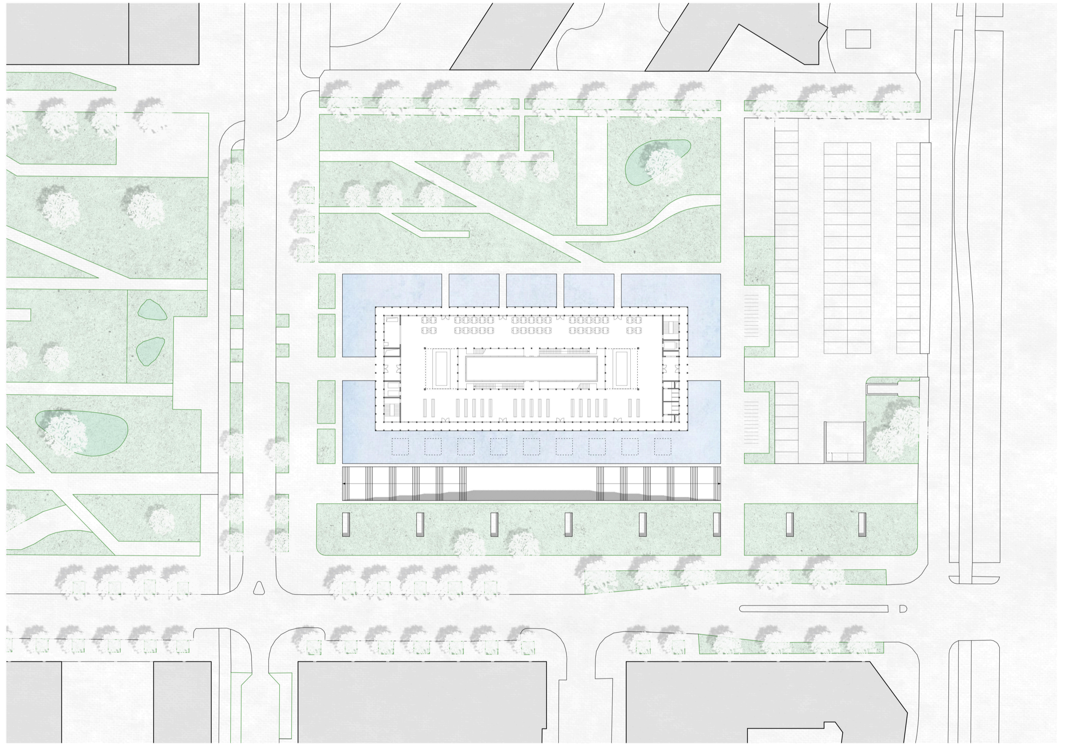
Site Plan with Ground Floor M 1:500
